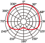
Figure 1: Polar pattern
