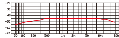
Figure 2: Frequency response
