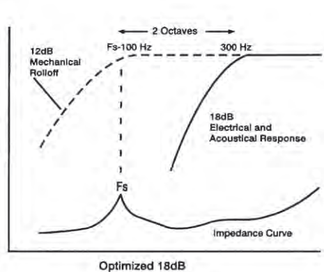
Optimized 6 & 18 dB Slope Selections
