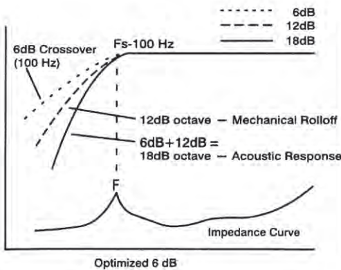
Optimized 6 & 18 dB Slope Selections
