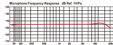
Figure 2: Frequency response
