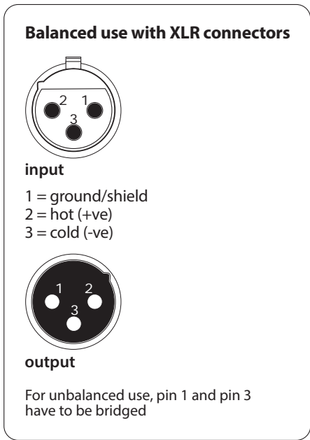
XLR connections
