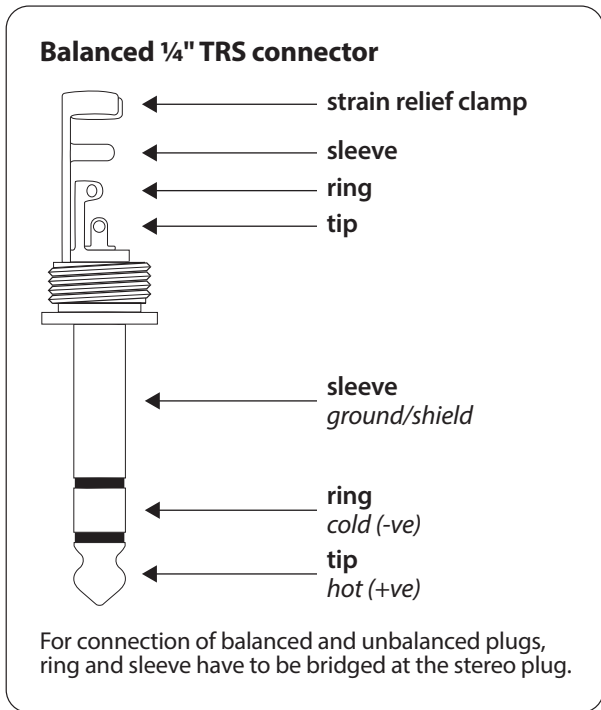
1/4" stereo plug
